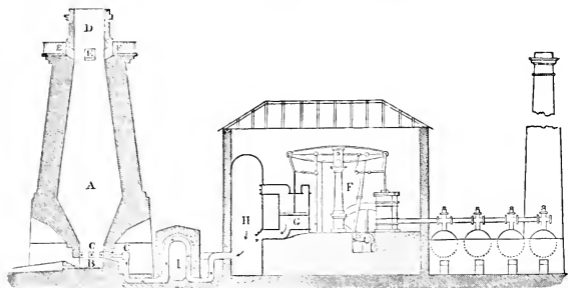
Fig. 1.—Hot Blast-furnace.
